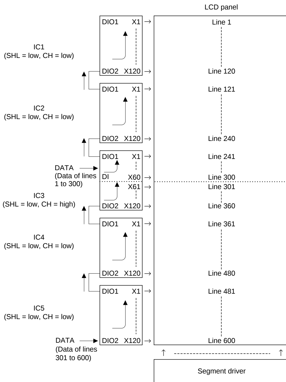
Figure 9 Dual-Screen Configuration of a 600-Line LCD Panel with a 1/300 Duty Cycle (2)
