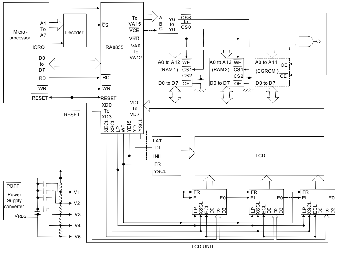
Figure 8-6: System Interconnection Diagram
